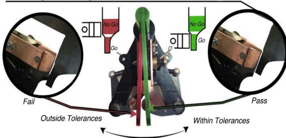
Main Moving Contact, Gauge-Go, No Go. Tool T85792
