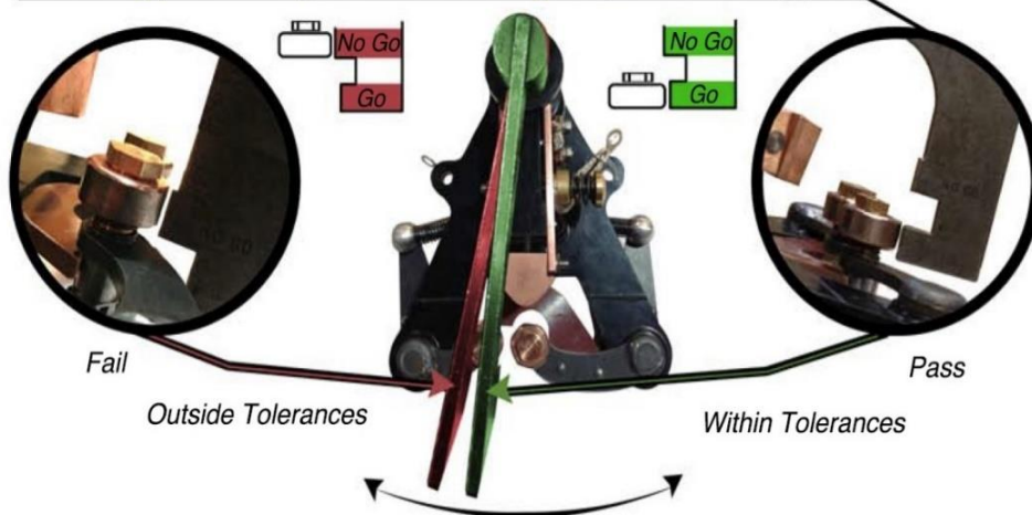
Main Moving Contact, Gauge-Go, No Go. Tool T85792
