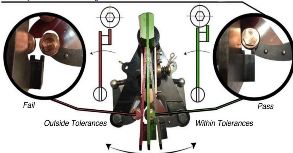
Main Arcing (Transitional), Roller Contact Gauge-Go, No Go. Tool MT87486
