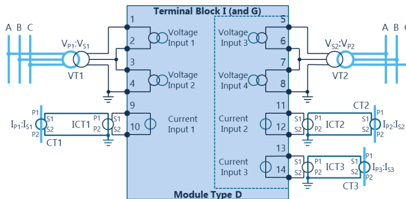
Figure 11 Typical connection diagram for AC input module (type D)
