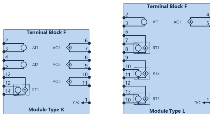
Figure 16 Terminal arrangements for DC analogue modules (type K and type L)
